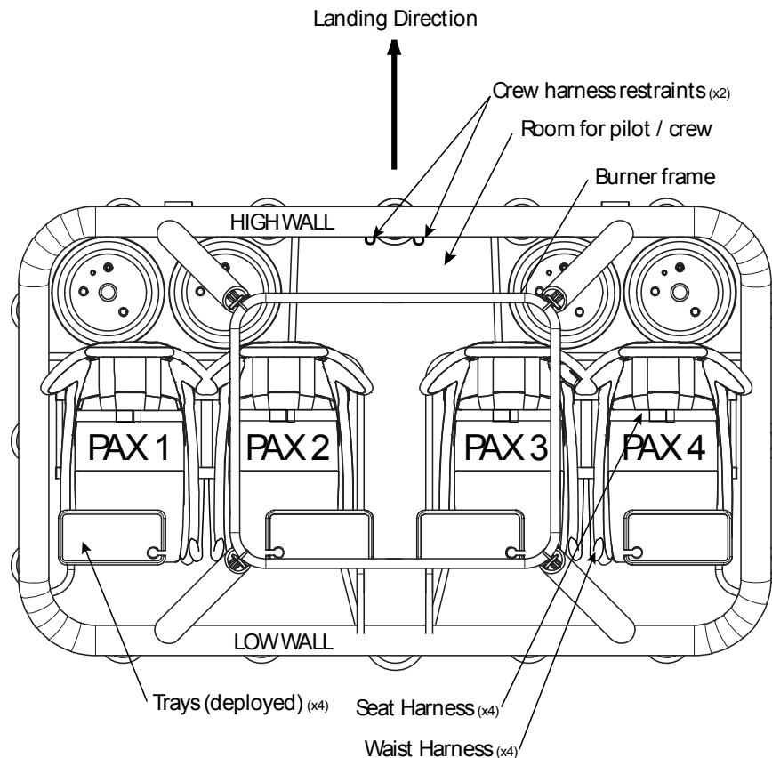
Top view of the VISTA 4 (CV-08 Basket) - (Burner not displayed) Trays to be stowed for landing.
